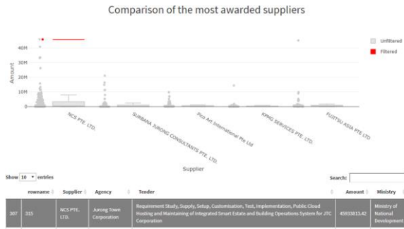
Figure 12. Scatterplot & Boxplot
